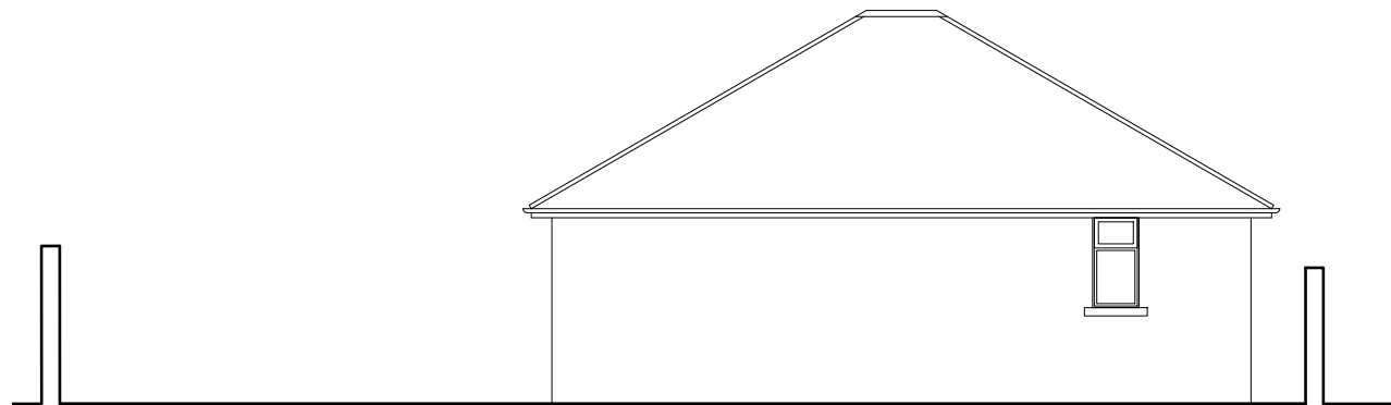
Existing Rear Elevation - 1:100
