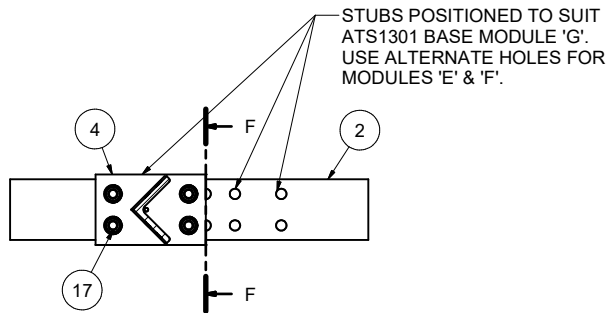
SECTION E-E
