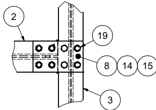
DETAIL C HAMMERHEAD CONNECTION DETAIL
