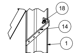
DETAIL N FEEDER BRACKET DETAIL
