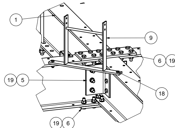
DETAIL H
