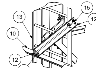
DETAIL G LADDER CONNECTION DETAIL
