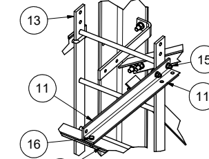
DETAIL F TOP LADDER CONNECTION DETAIL
