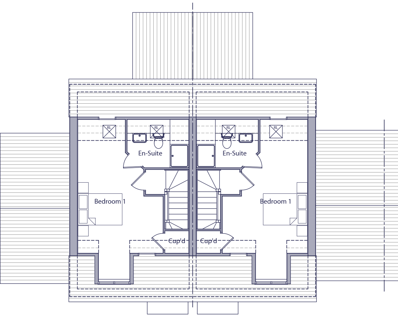
SECOND FLOOR PLAN PLOT 4042
