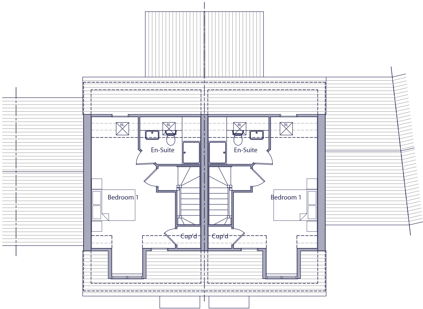
SECOND FLOOR PLAN PLOT 4092
