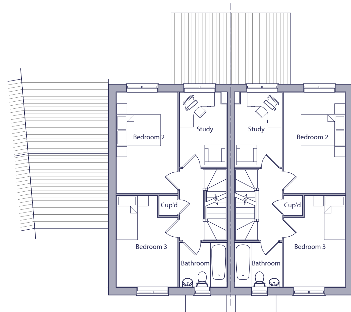
FIRST FLOOR PLAN PLOT 4101
