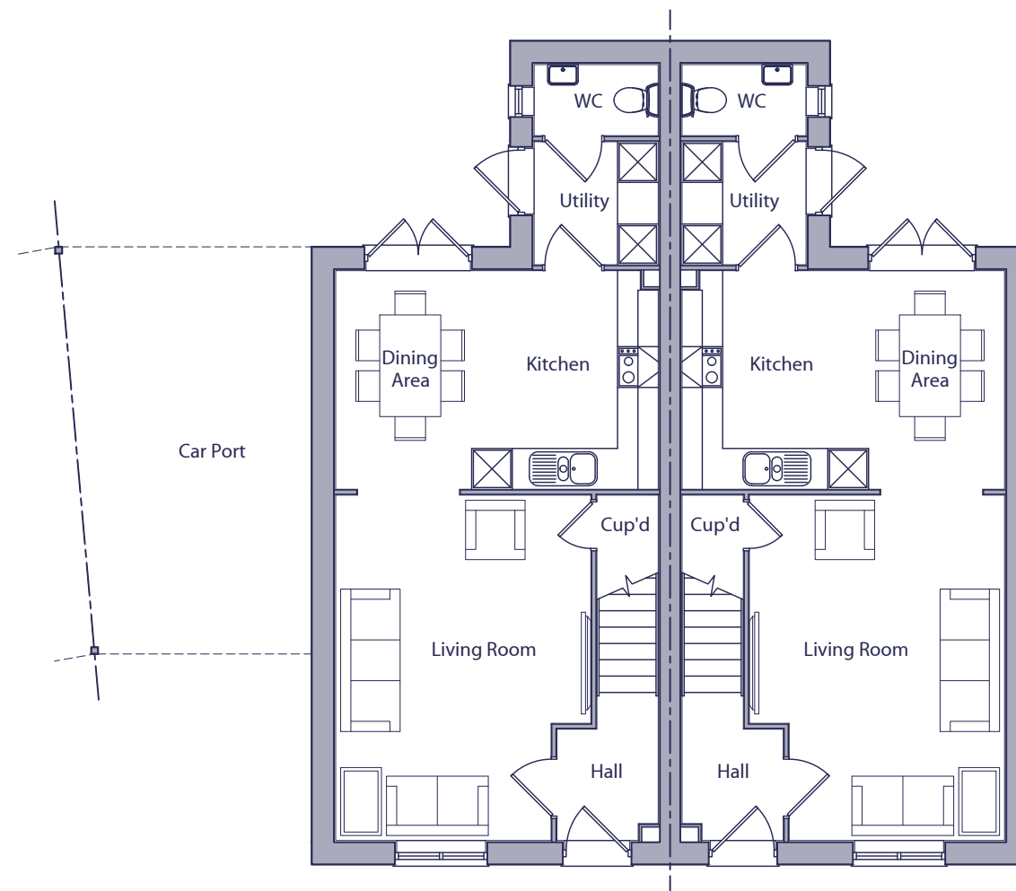
GROUND FLOOR PLAN PLOT 4101
