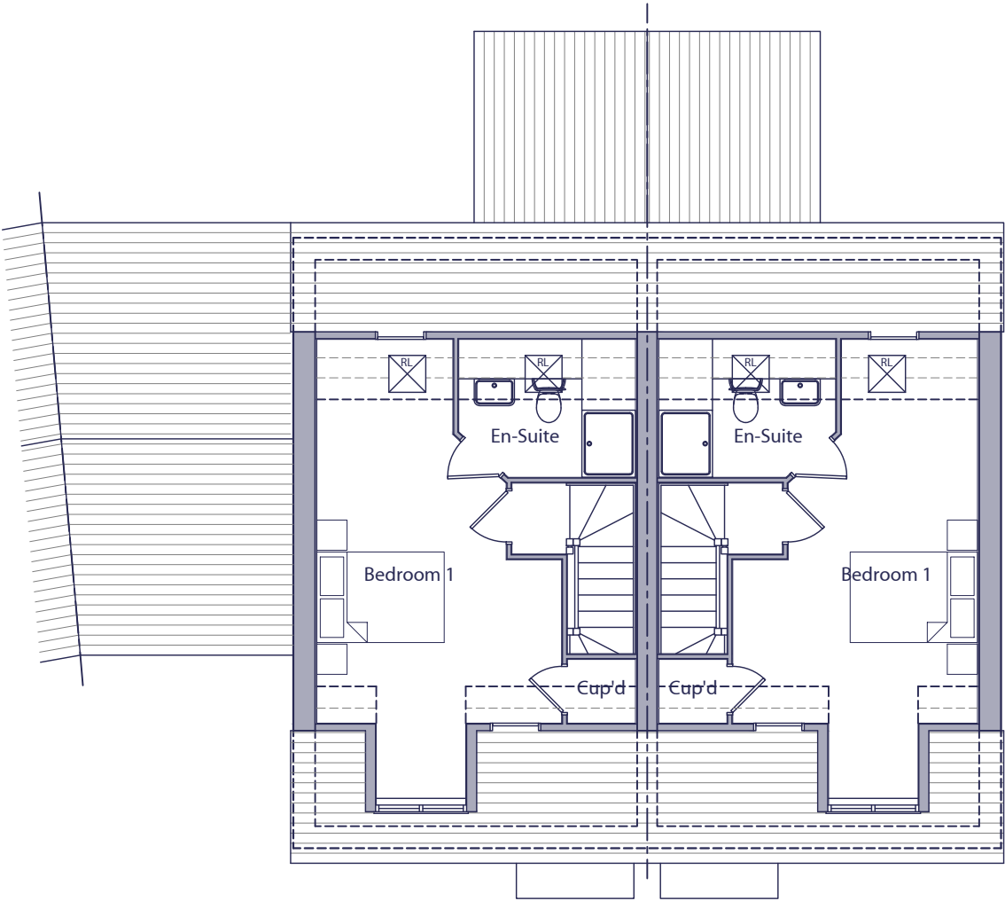
SECOND FLOOR PLAN PLOT 4101
