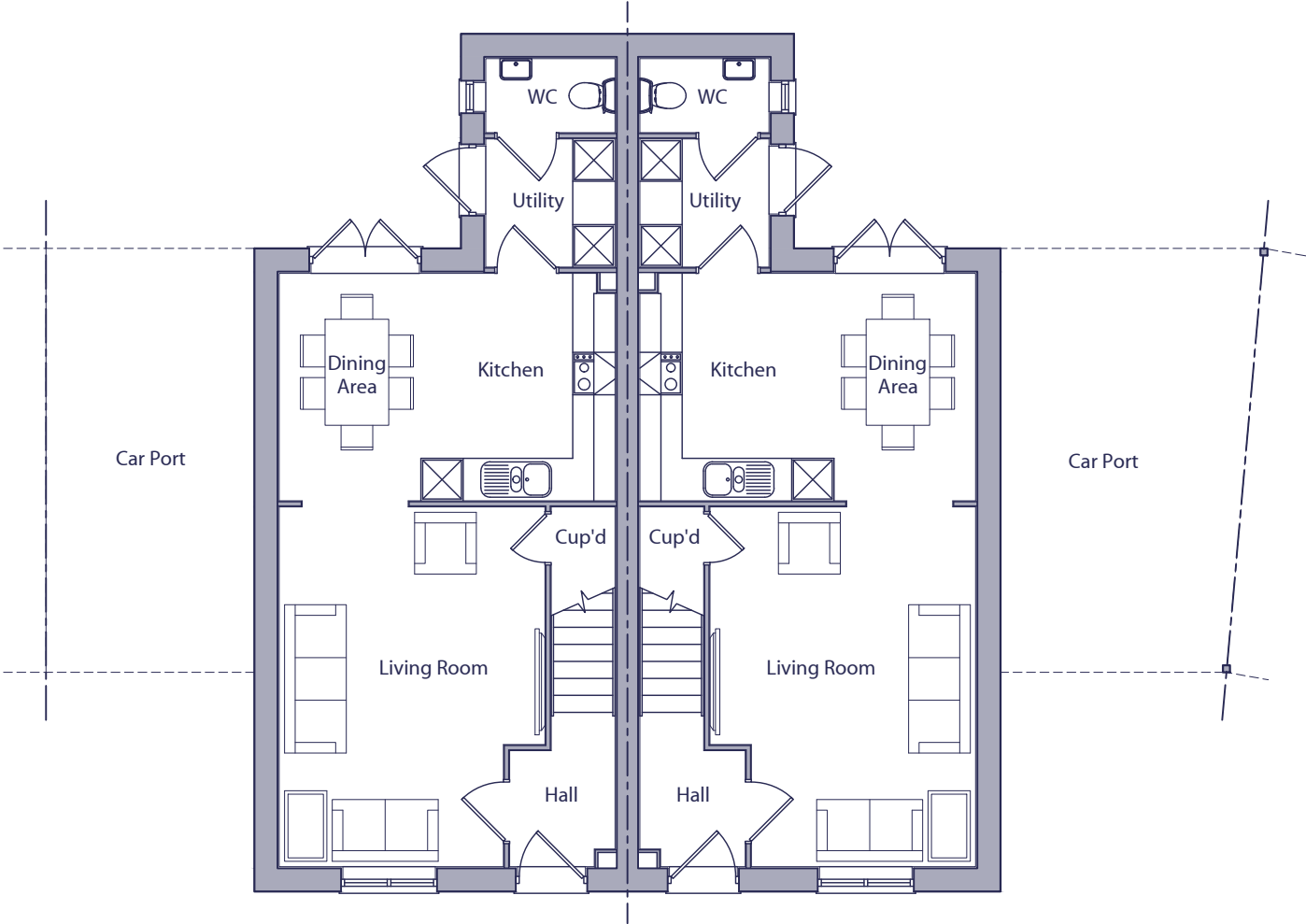
GROUND FLOOR PLAN PLOT 4103
