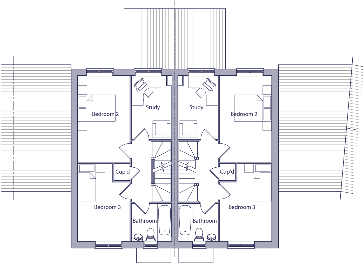
FIRST FLOOR PLAN PLOT 4103
