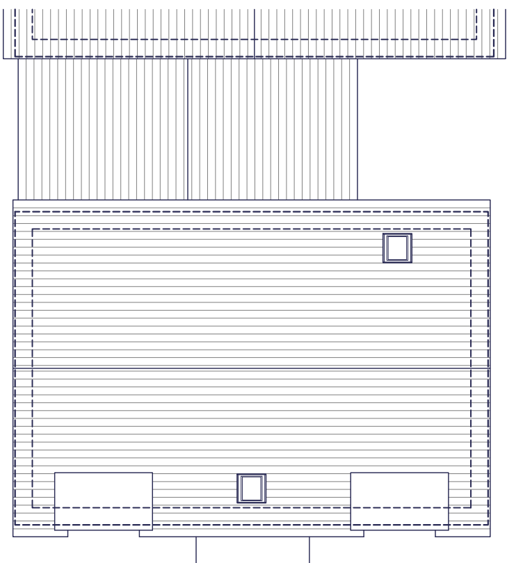
ROOF PLAN
