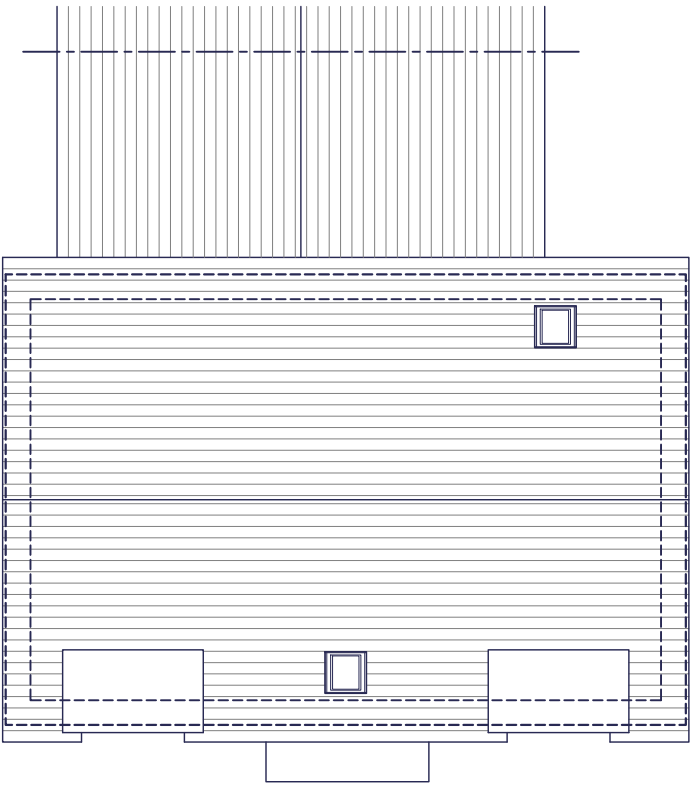
ROOF PLAN
