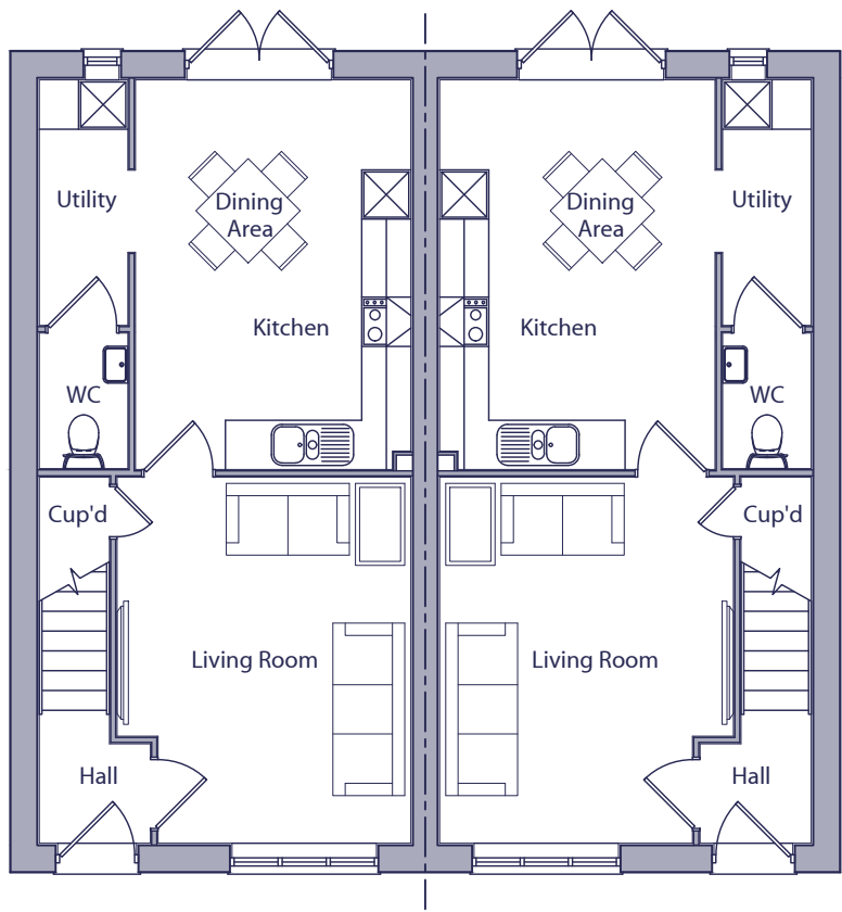
GROUND FLOOR PLAN PLOT 3036 PLOT 4026 PLOT 3037 PLOT 4025
