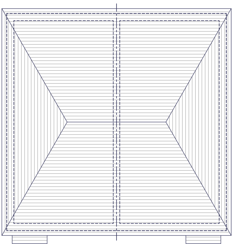
ROOF PLAN PLOT 3012 PLOT 3013 PLOT 3032 PLOT 3033
