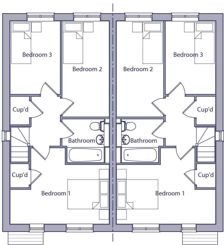
FIRST FLOOR PLAN PLOT 3012 PLOT 3013 PLOT 3032 PLOT 3033
