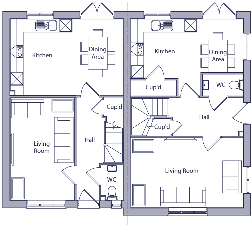
GROUND FLOOR PLAN L358 TYPE - PLOT 3040 L360 TYPE - PLOT 3041
