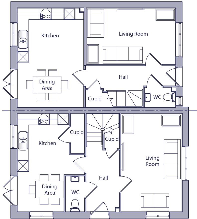
L358 TYPE - PLOT 3015
