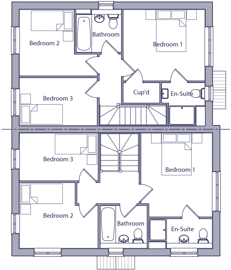
FIRST FLOOR PLAN L360 TYPE - PLOT 3014
