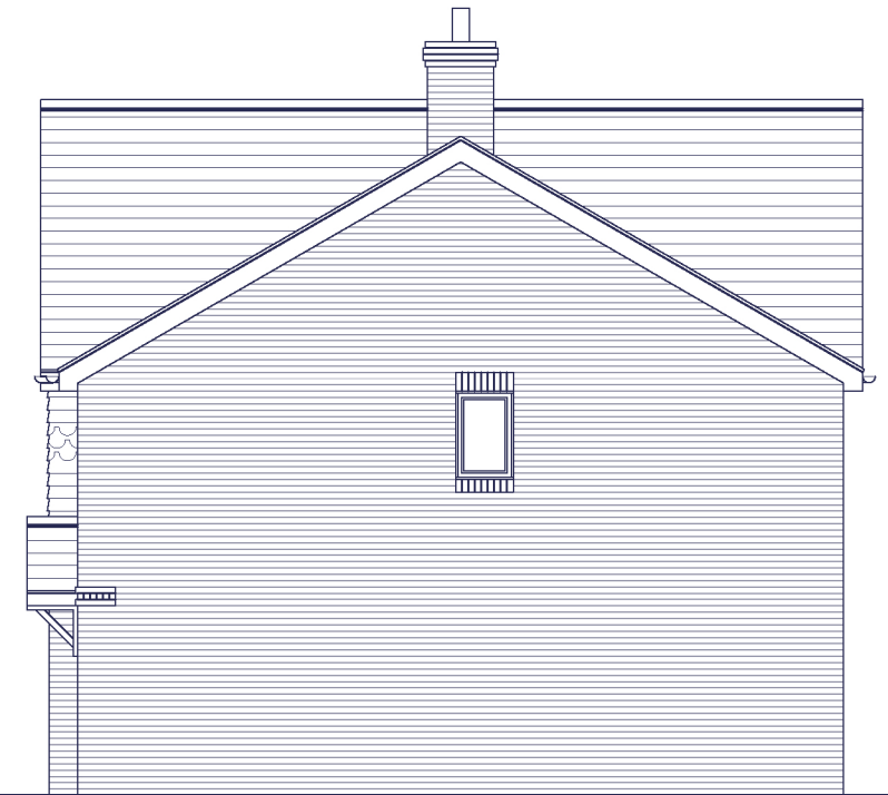
SIDE ELEVATION L358 TYPE PLOT 3015
