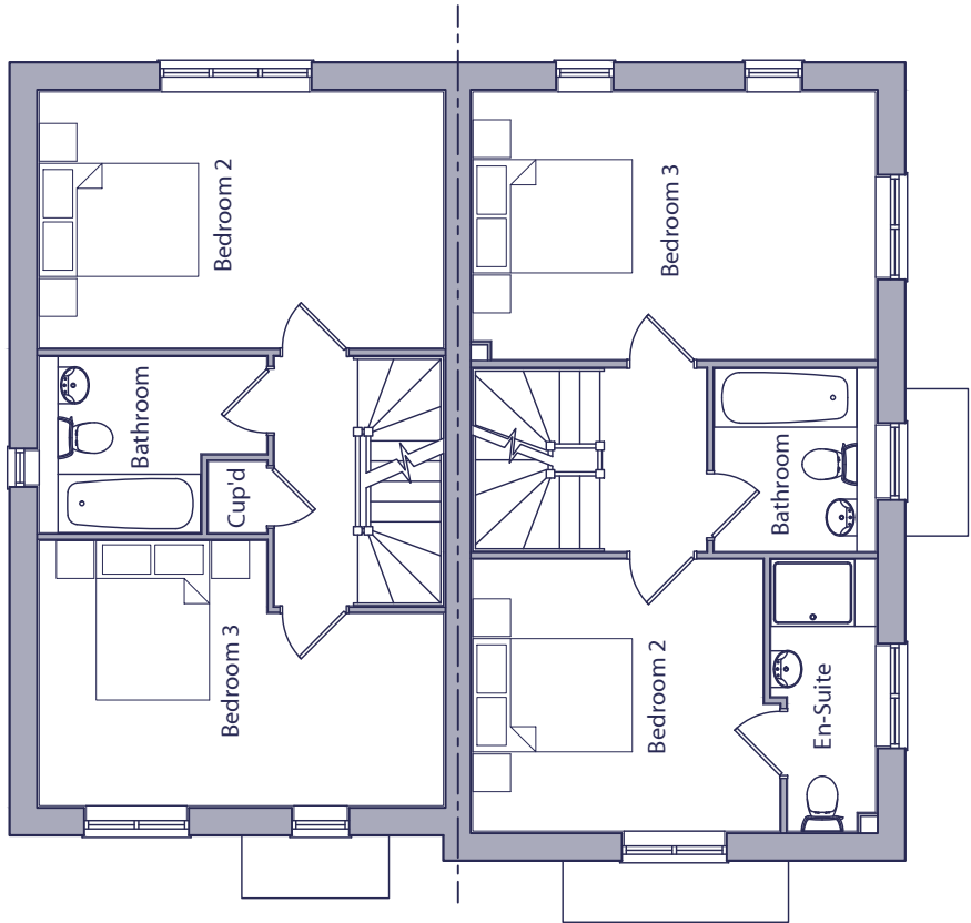
FIRST FLOOR PLAN L367 TYPE - PLOT 3002
