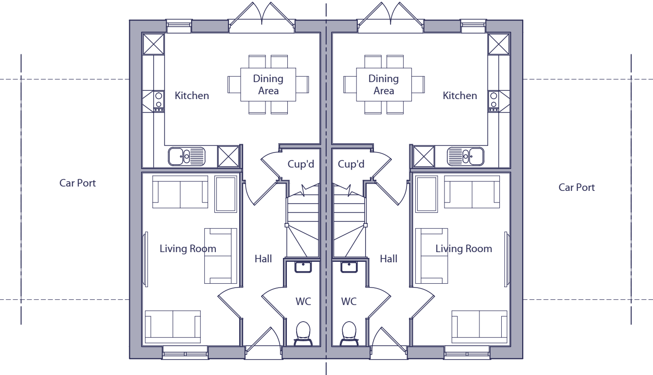
GROUND FLOOR PLAN PLOT 3068, 3070, 3072 & 3074
