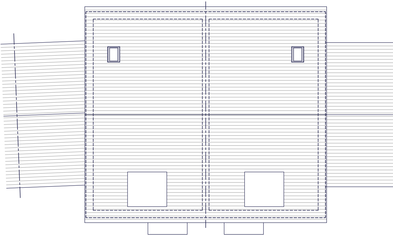
ROOF PLAN PLOT 3076
