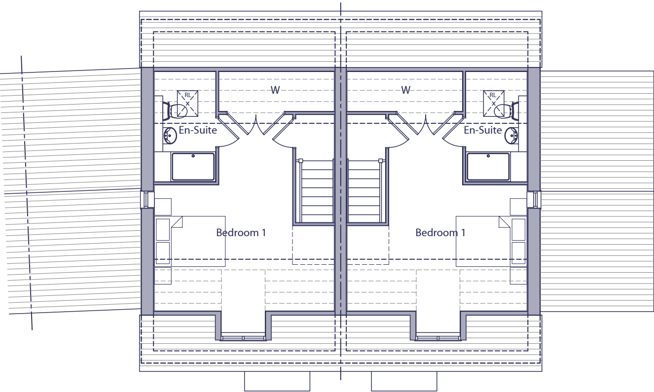
SECOND FLOOR PLAN PLOT 3076
