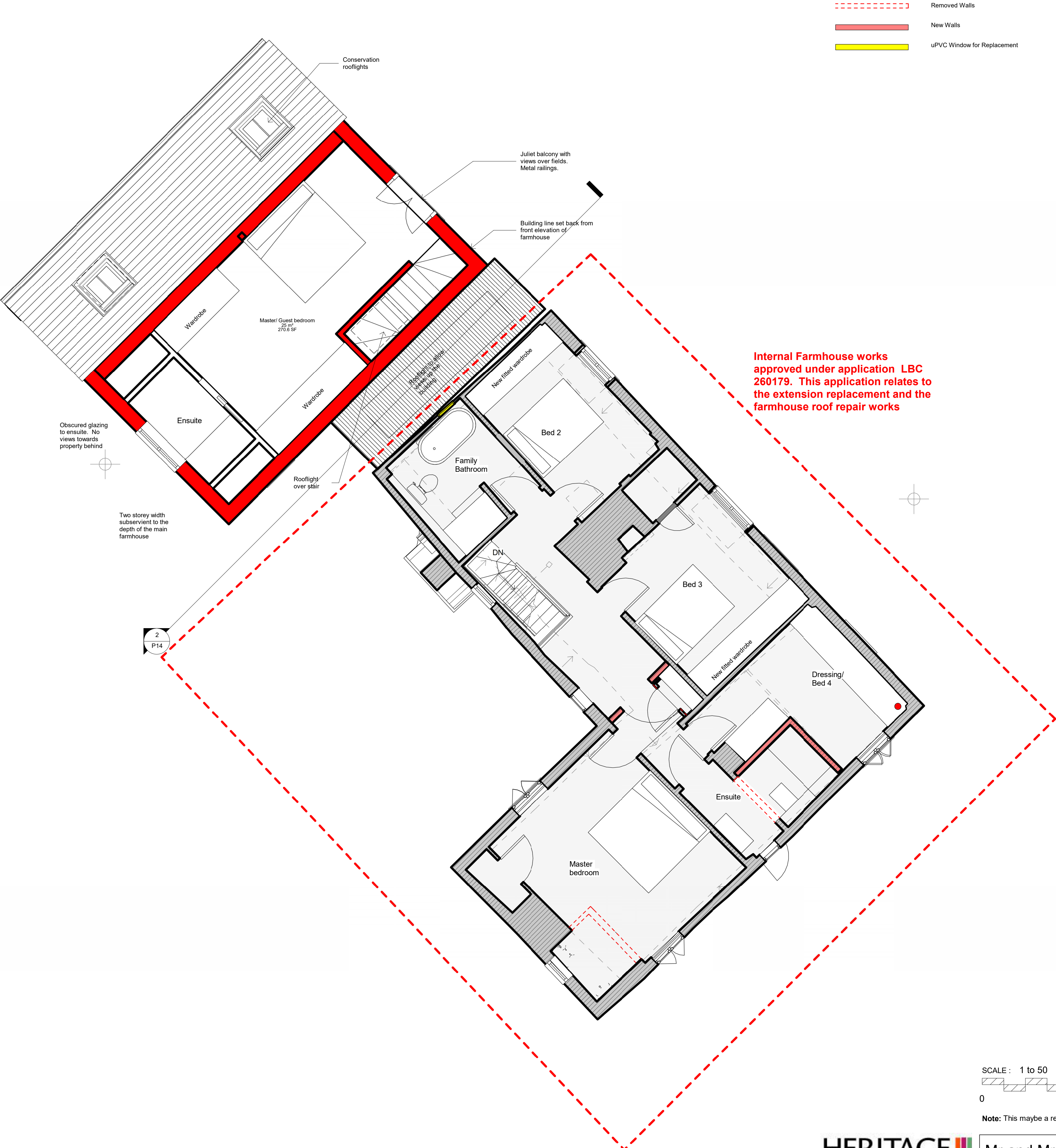
1st Floor Proposed 1 : 50
