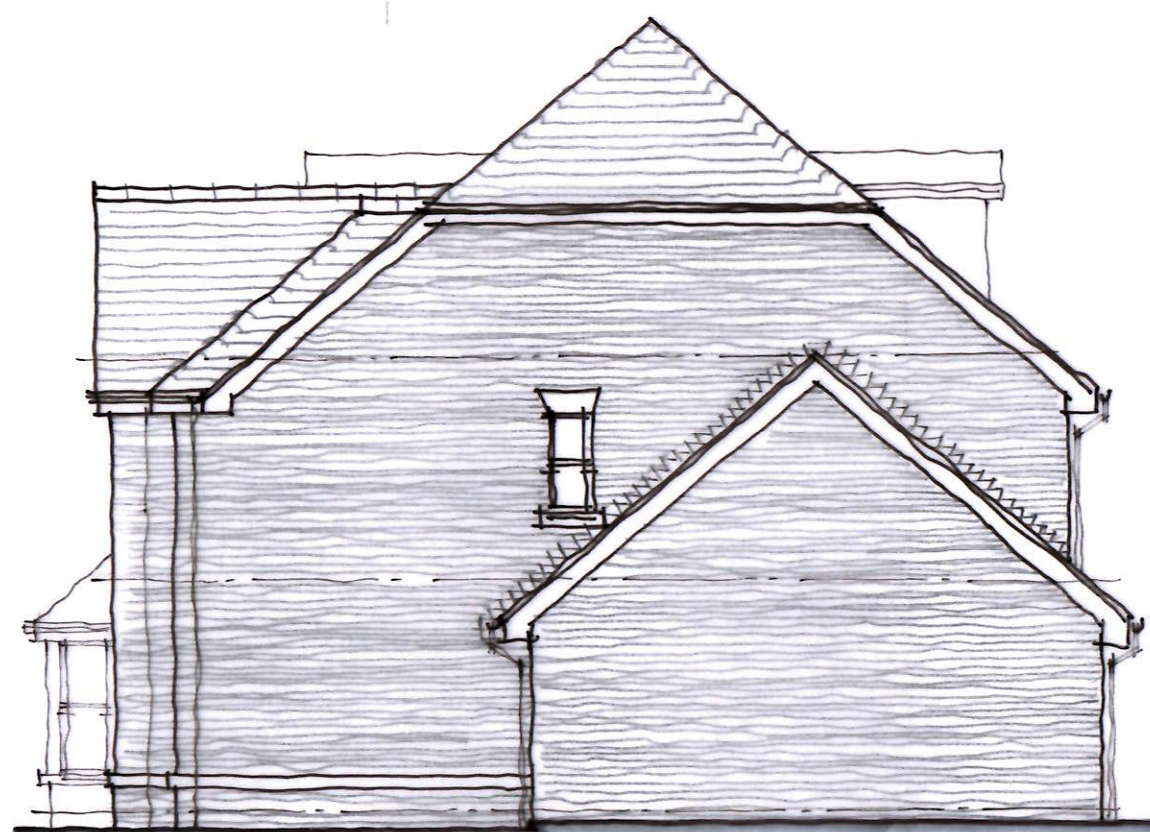
Rear Elevation Plot 4 Handed, Plot 5 As Drawn
