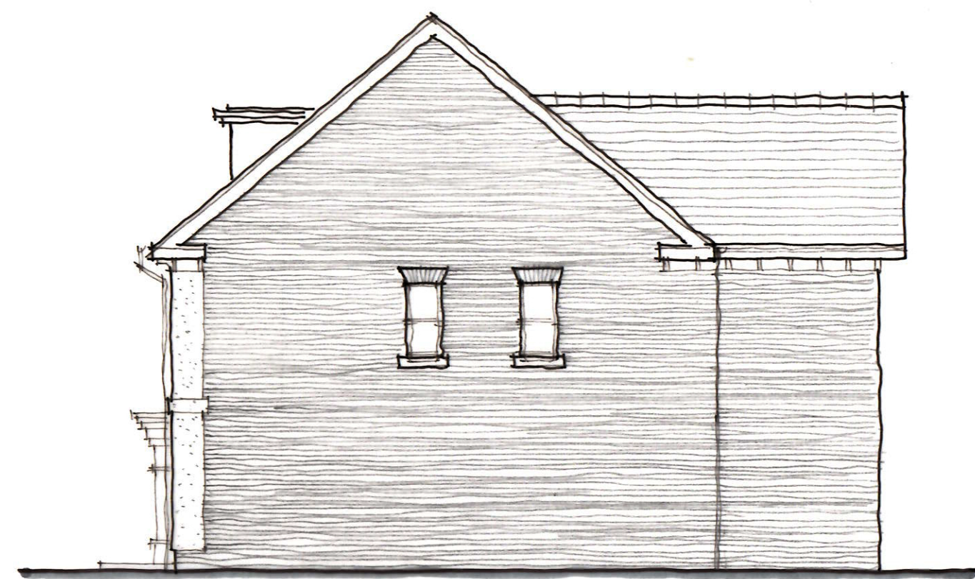
Side Elevation Plots 7 and 8 As Drawn
