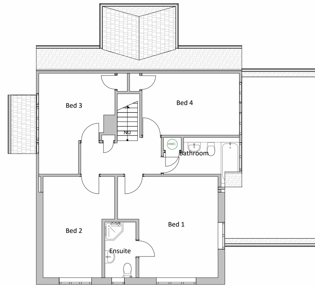
② Existing First Floor_72sqm 1 : 100
