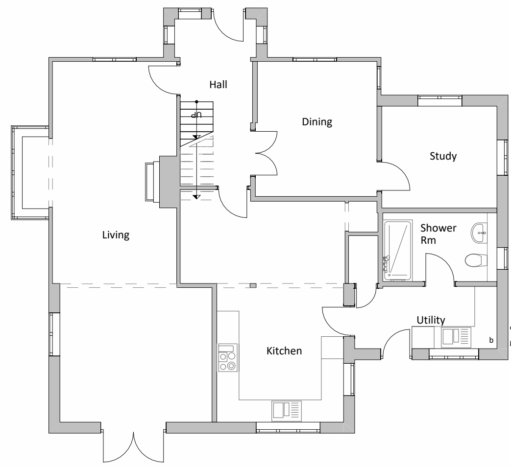
① Existing Ground Floor_108sqm 1 : 100
