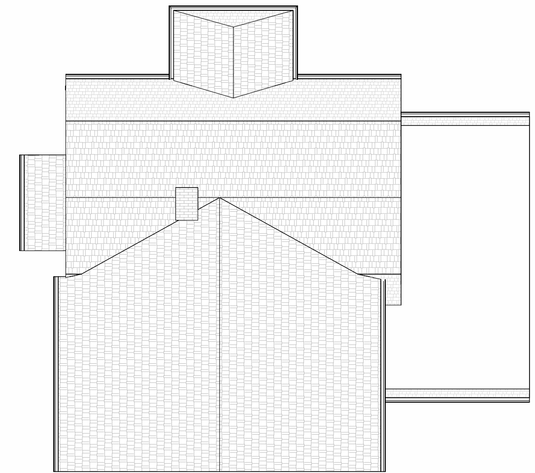
③ Existing Roof Plan 1 : 100
