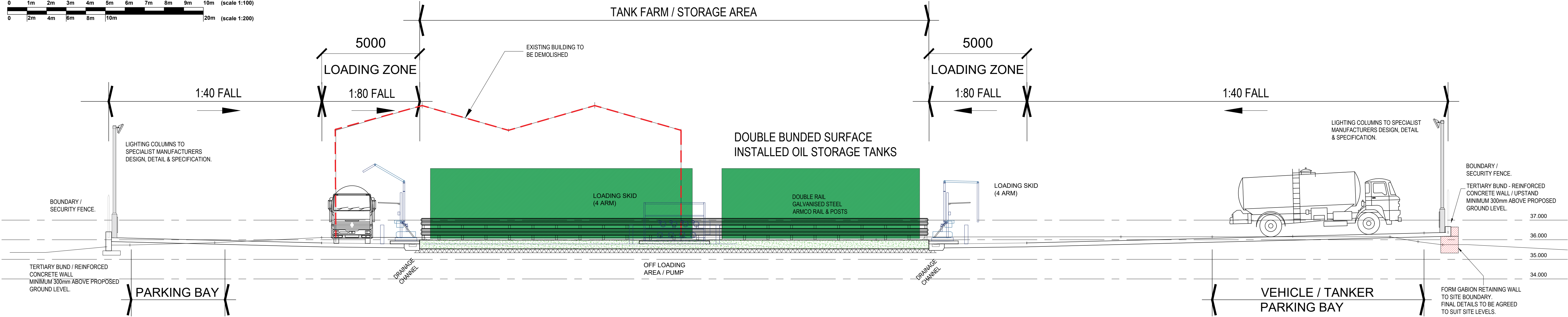
PROPOSED CROSS SECTION - THROUGH SITE (SCALE 1:100)
