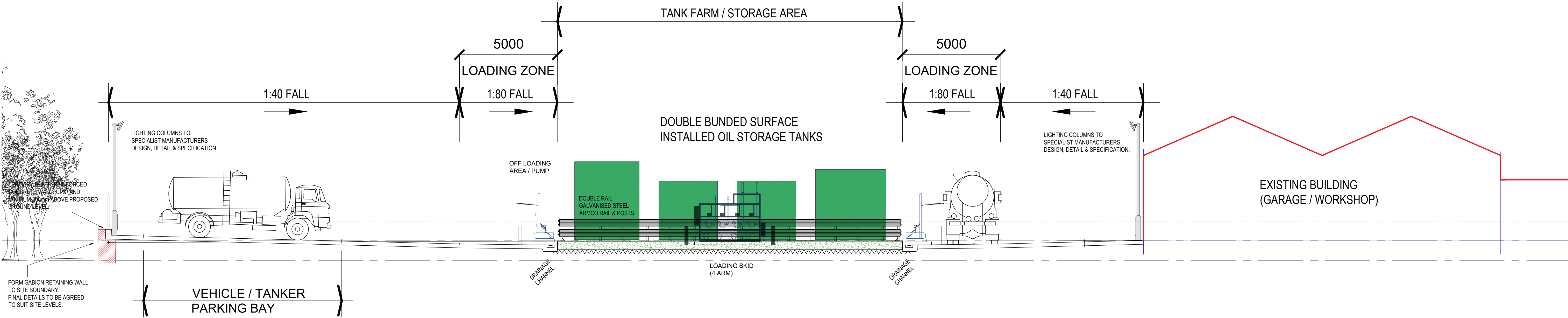
PROPOSED LONGITUDINAL SECTION - THROUGH SITE (SCALE 1:100)
