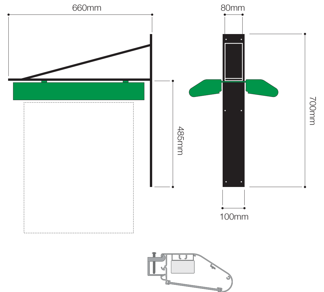
Troughlight Profile
