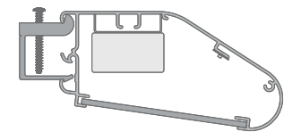
Troughlight Profile
