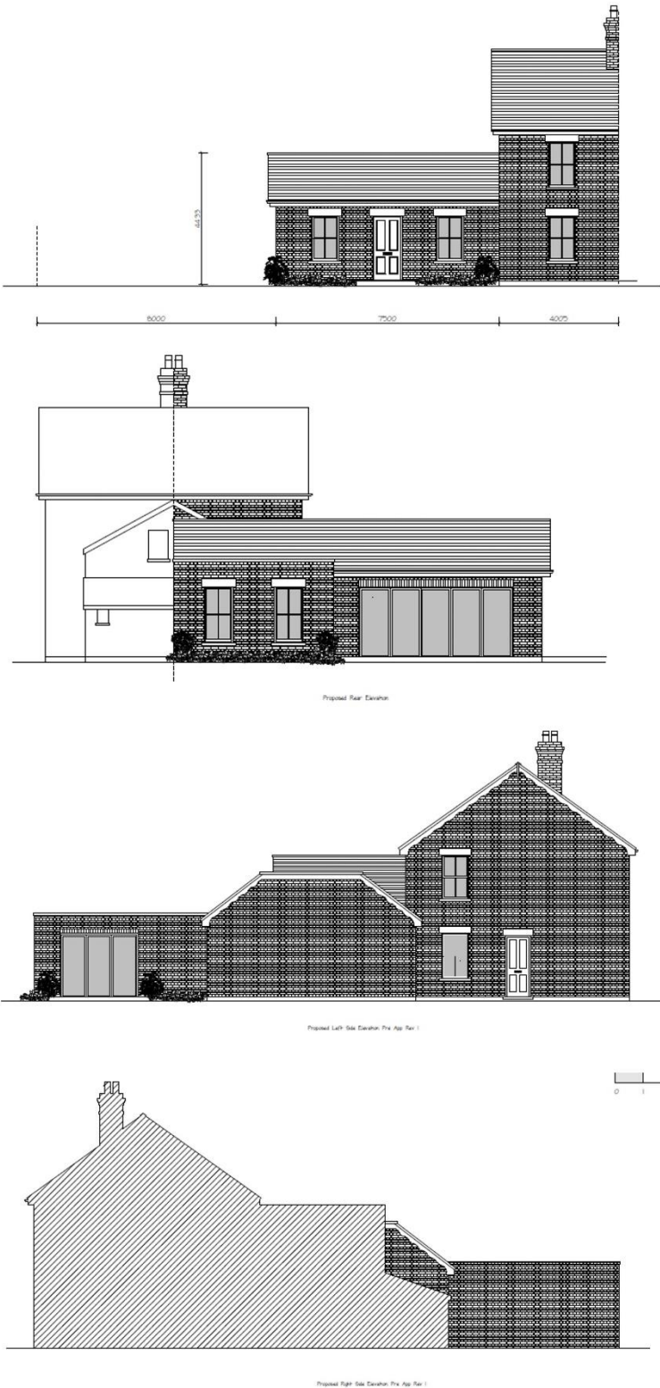
Figure 2 – Proposed elevations
