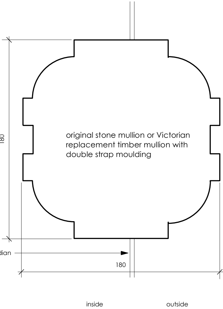
Stone casement and fixed light central mullion Detail B
