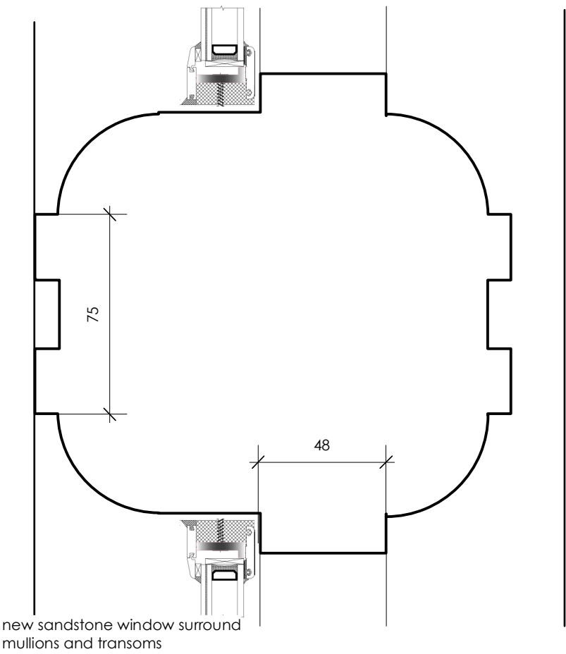
central mullion plan section
