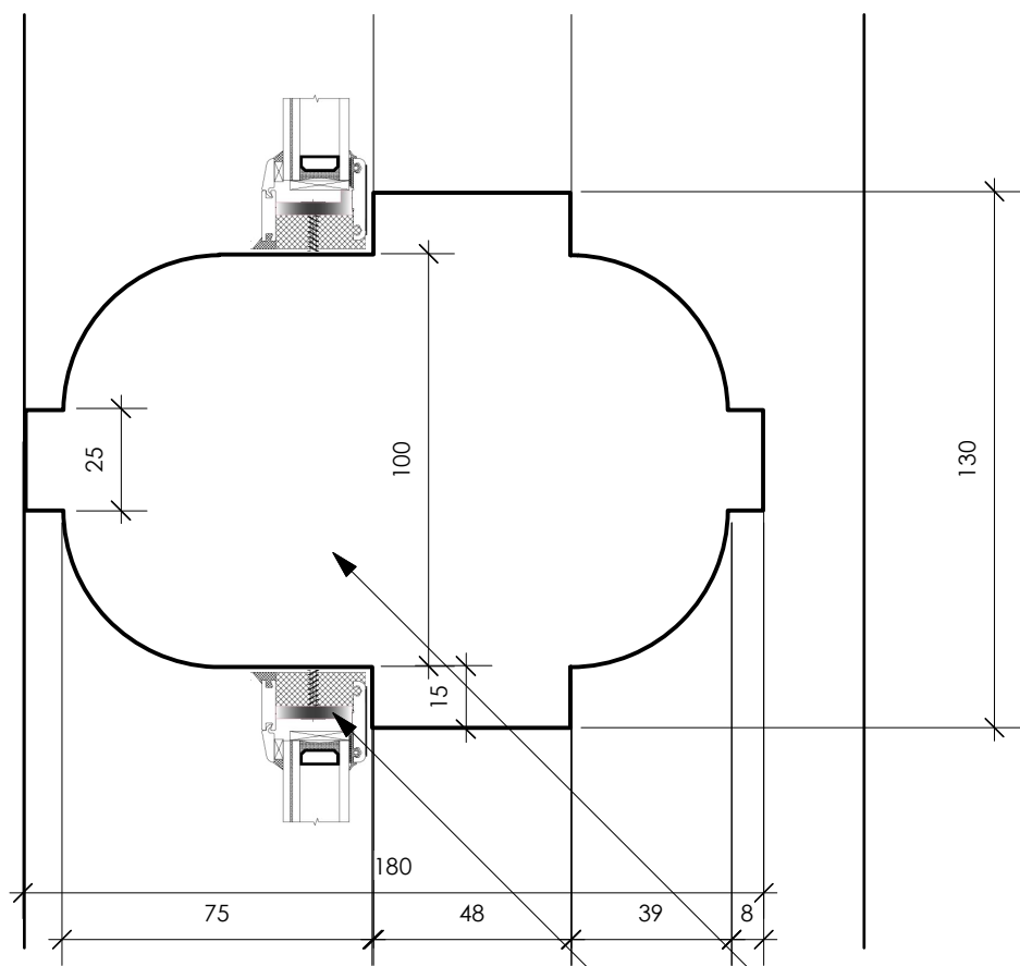
intermediary mullion plan section
