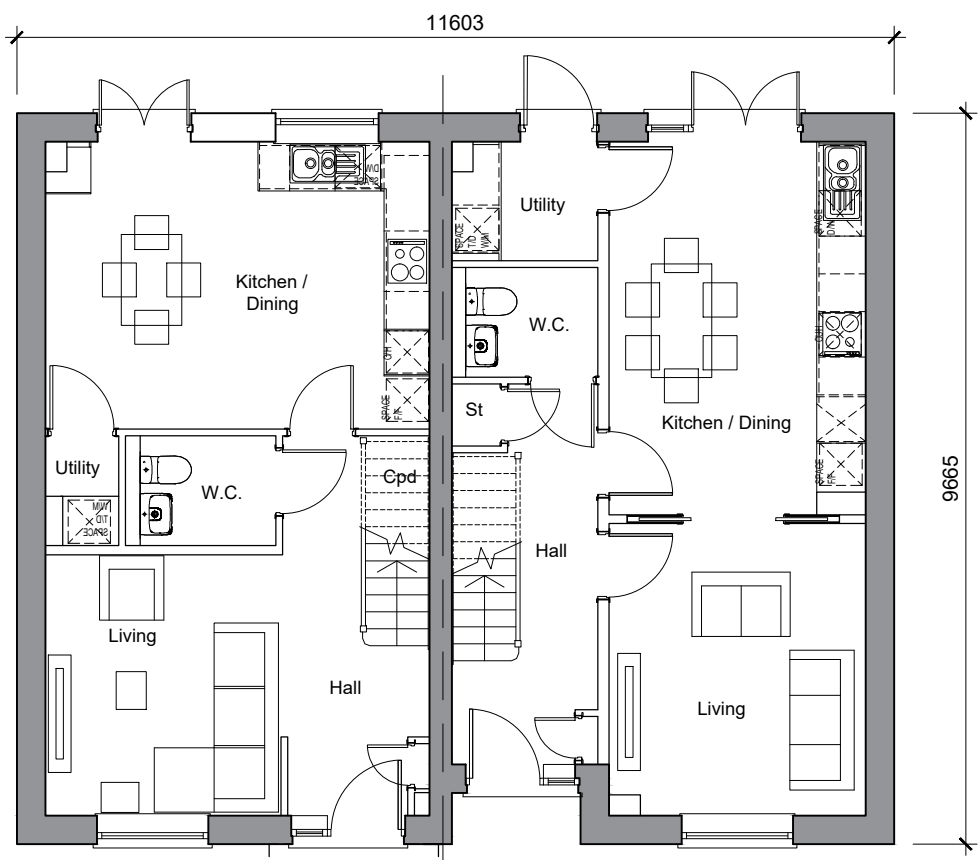
PH3B - 3 Bedroom House NIA 90.27sqm Ground Floor Plan Plots 28-29 PH3A - 3 Bedroom House NIA 94.54sqm
