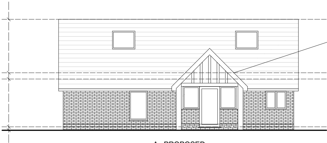
As PROPOSED
