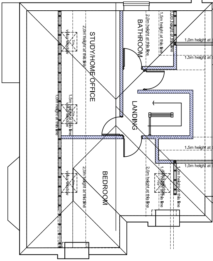
Roof Floor Plan
