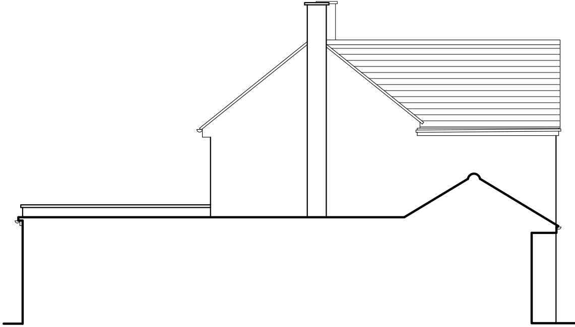
SIDE ELEVATION 1:100
