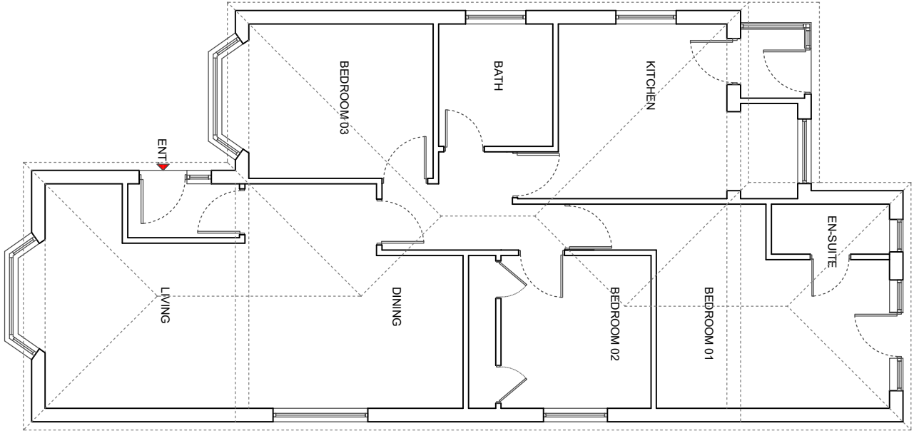
GROUND FLOOR PLAN AS EXISTING 108 READING ROAD, WOODLEY RG5 3AD
