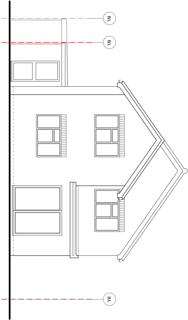
REAR ELEVATION AS PRE-EXISTING
