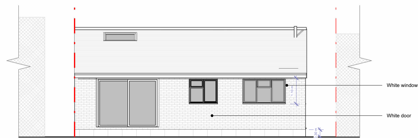
Rear Elevation
