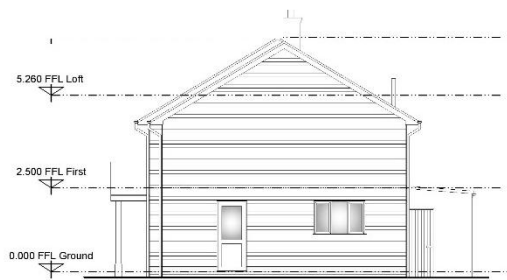
Proposed South Elevation Scale 1:100
