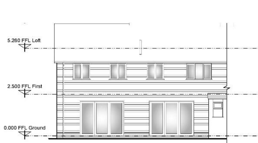
Proposed West Elevation Scale 1:100
