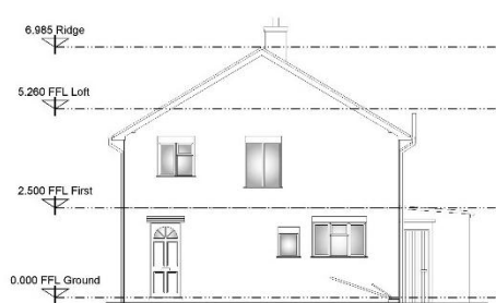
Existing South Elevation Scale 1:100
