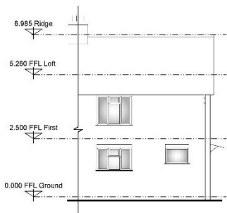
Existing West Elevation Scale 1:100
