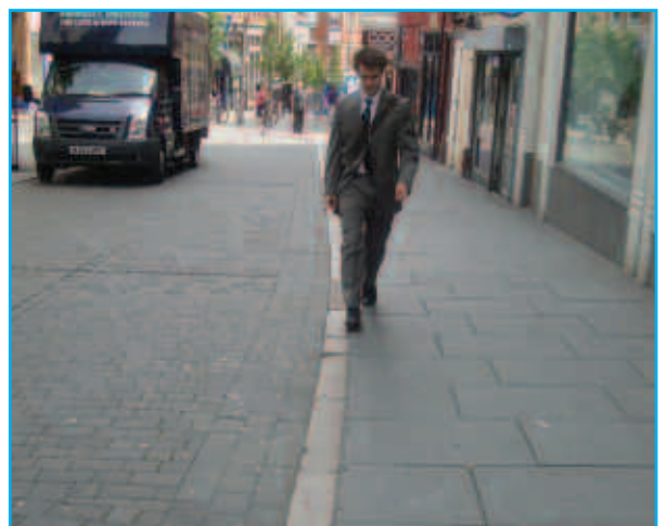
Kerb heights of between 75mm and zero (at informal crossings) were used with streetscape improvements in the centre of Nottingham.
