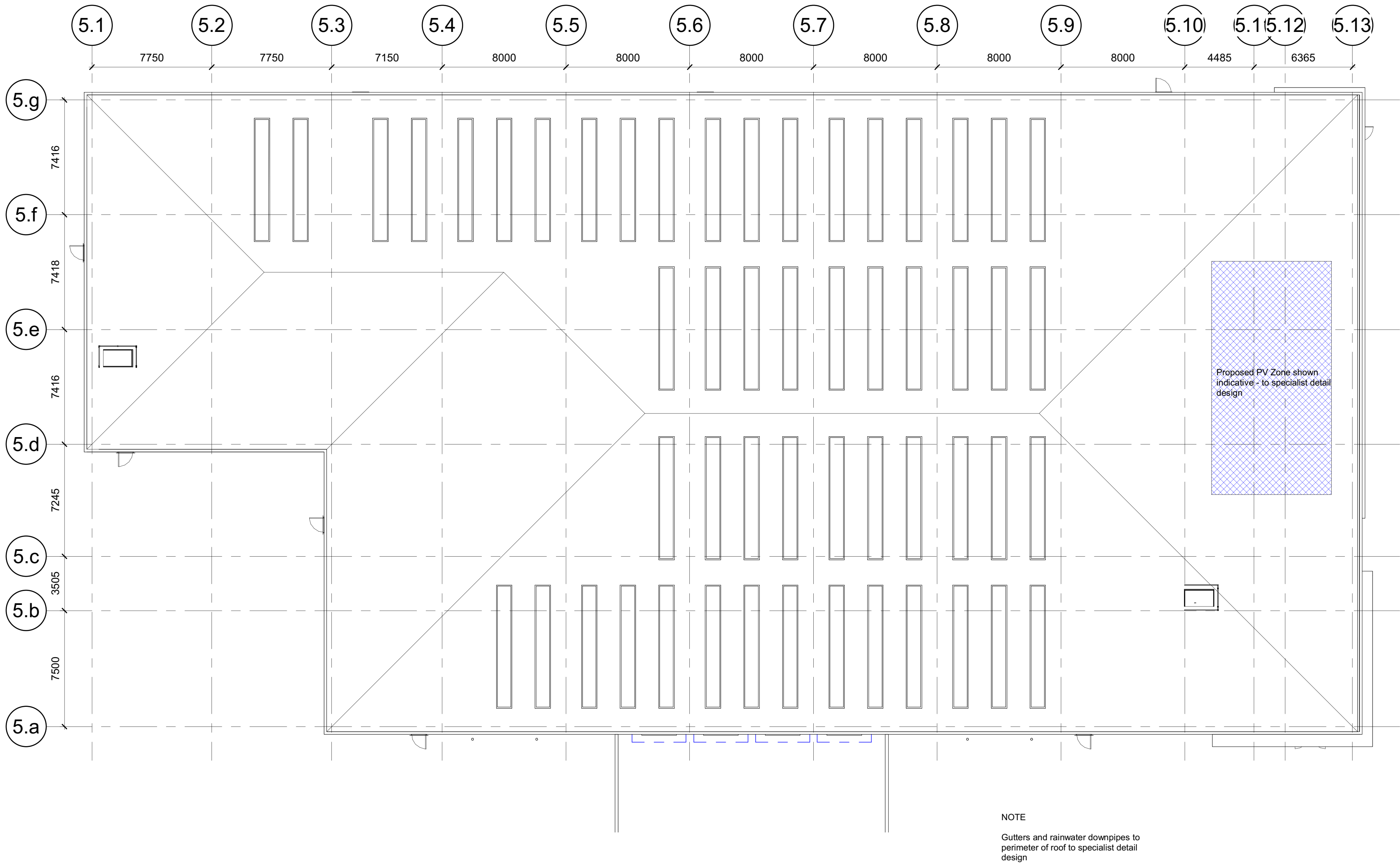
1 UNIT 5 - ROOF GA PLAN 1 : 200
