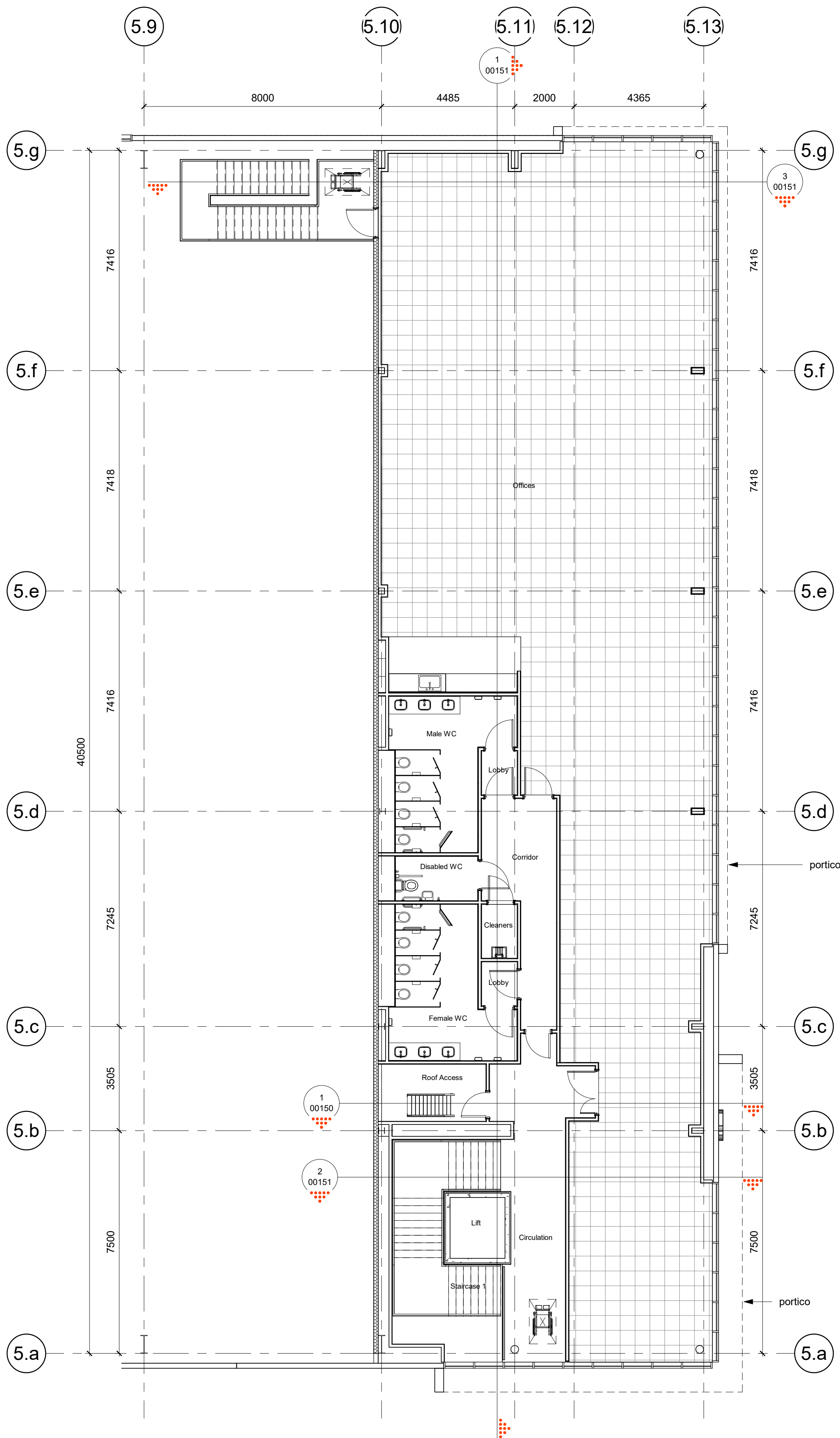
1 FIRST FLOOR OFFICE GA PLAN 1 : 100
