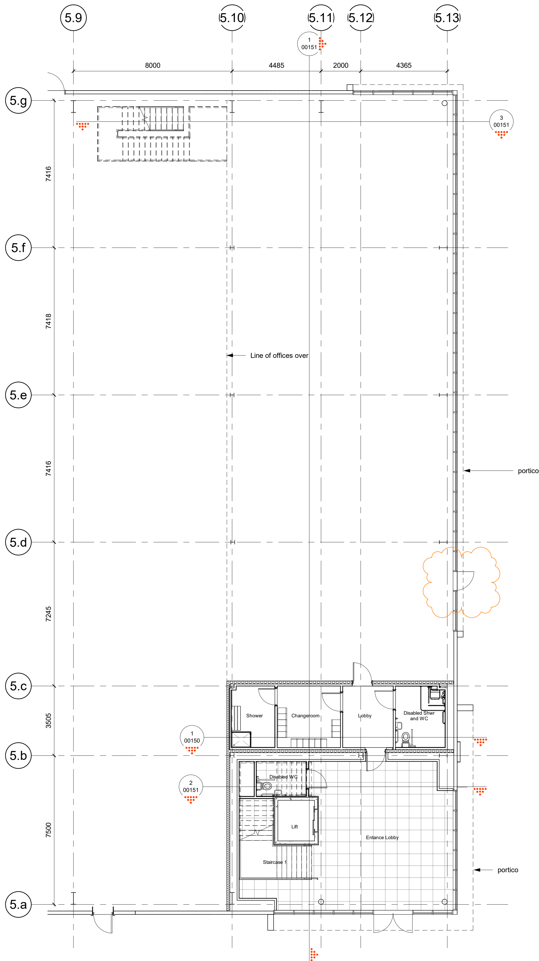
2 GROUND FLOOR OFFICE GA PLAN 1 : 100
