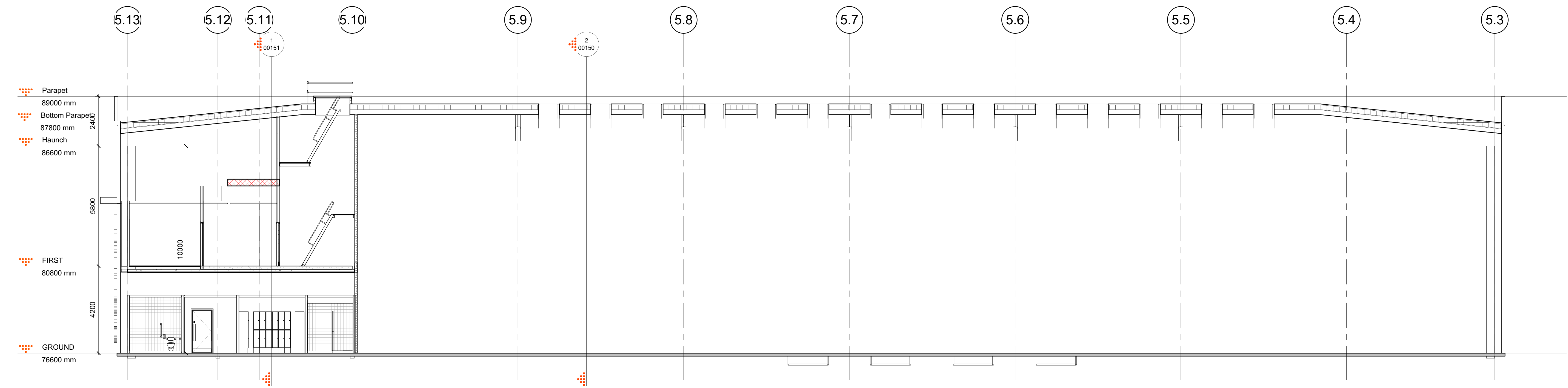
1 WAREHOUSE SECTION A 1 : 100
