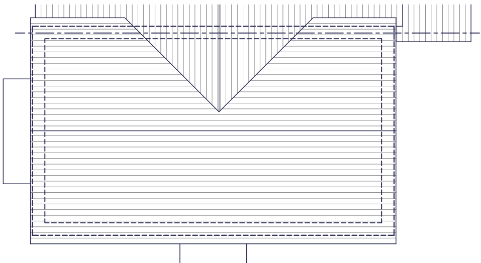
ROOF PLAN
