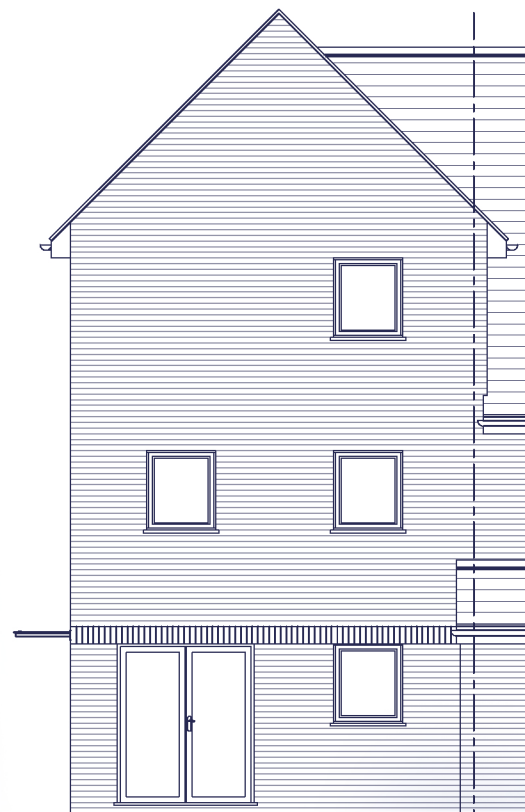
SIDE ELEVATION
