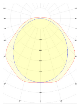
Luminaire Polar Intensity Diagram
