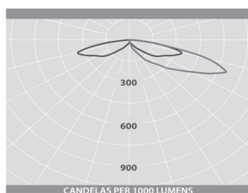
Luminaire Polar Intensity Diagram
