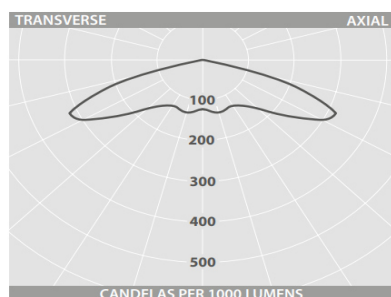
Luminaire Polar Intensity Diagram
