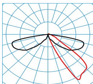
Luminaire Polar Intensity Diagram
