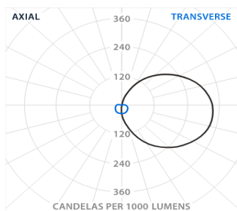
Luminaire Polar Intensity Diagram
