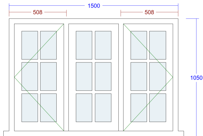
5. Flush Casement Window (W5 - Bathroom/Hall)
