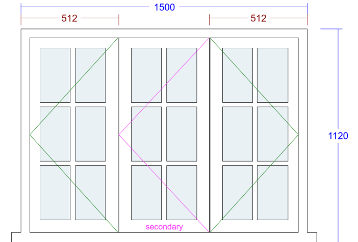
12. Conventional Cottage Window (W12 - Kitchen )
