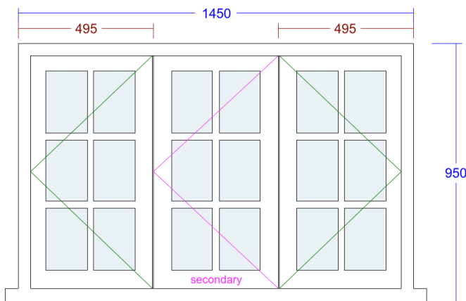
4. Conventional Cottage Window (W4 - Bedroom 2)
