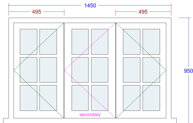
2. Conventional Cottage Window (W2 - Bedroom 1)
