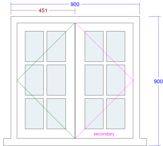
8. Conventional Cottage Window (W8 - Office)
