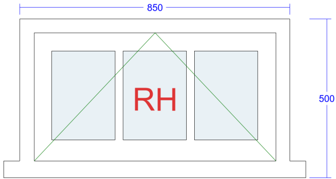
7. Conventional Cottage Window (W7 - Office)
