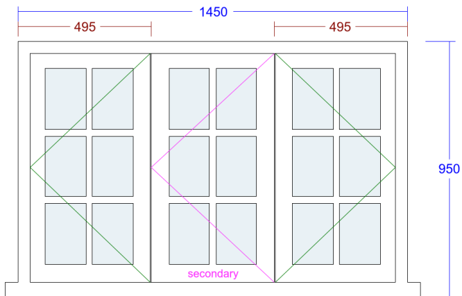
10. Conventional Cottage Window (W10 - Living Room)
