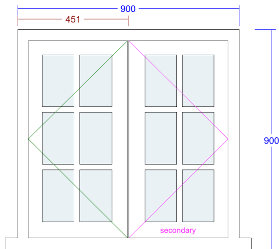
1. Conventional Cottage Window (W1 - Bedroom 3 (Dormer))
