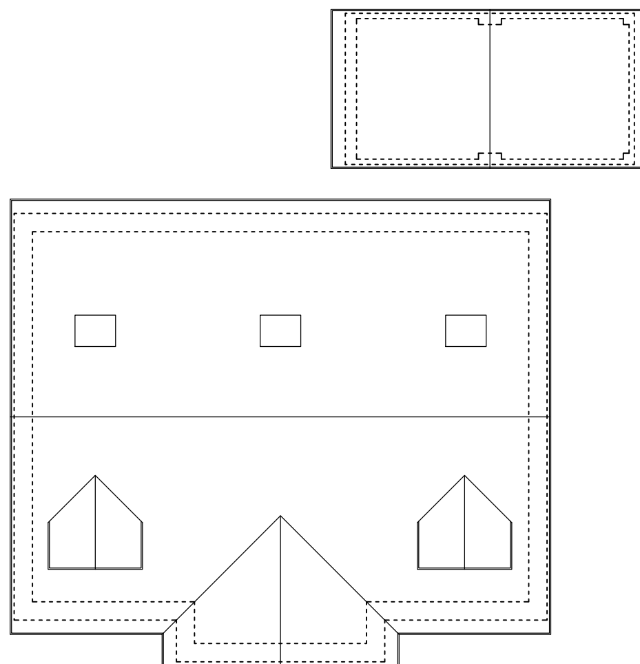
Roof Plan
