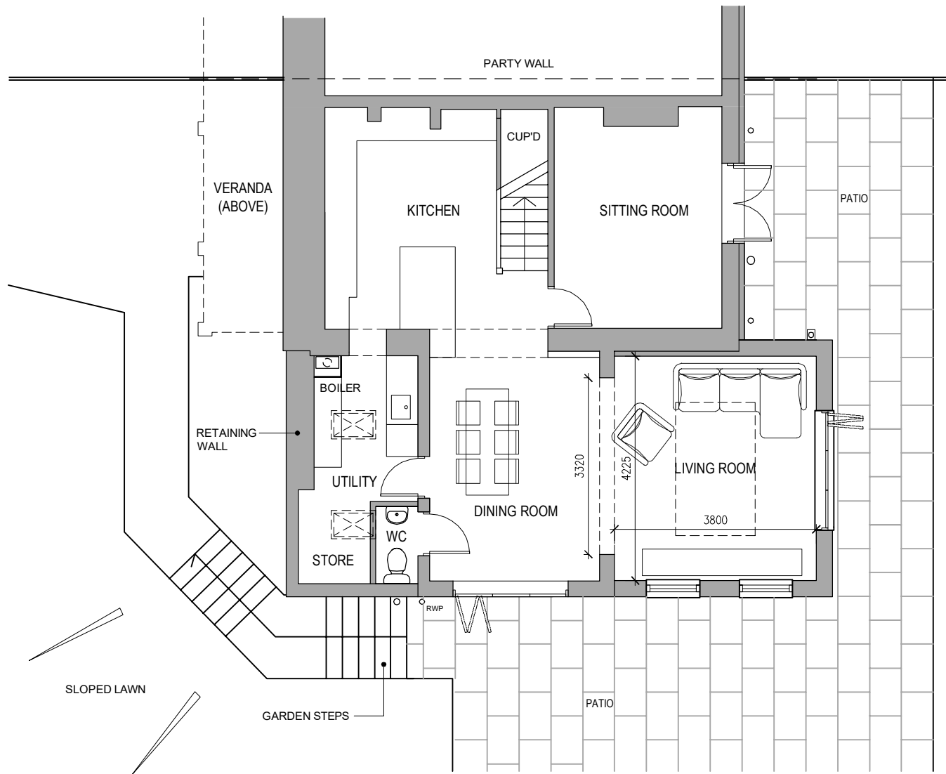
PROPOSED LOWER GROUND FLOOR PLAN
