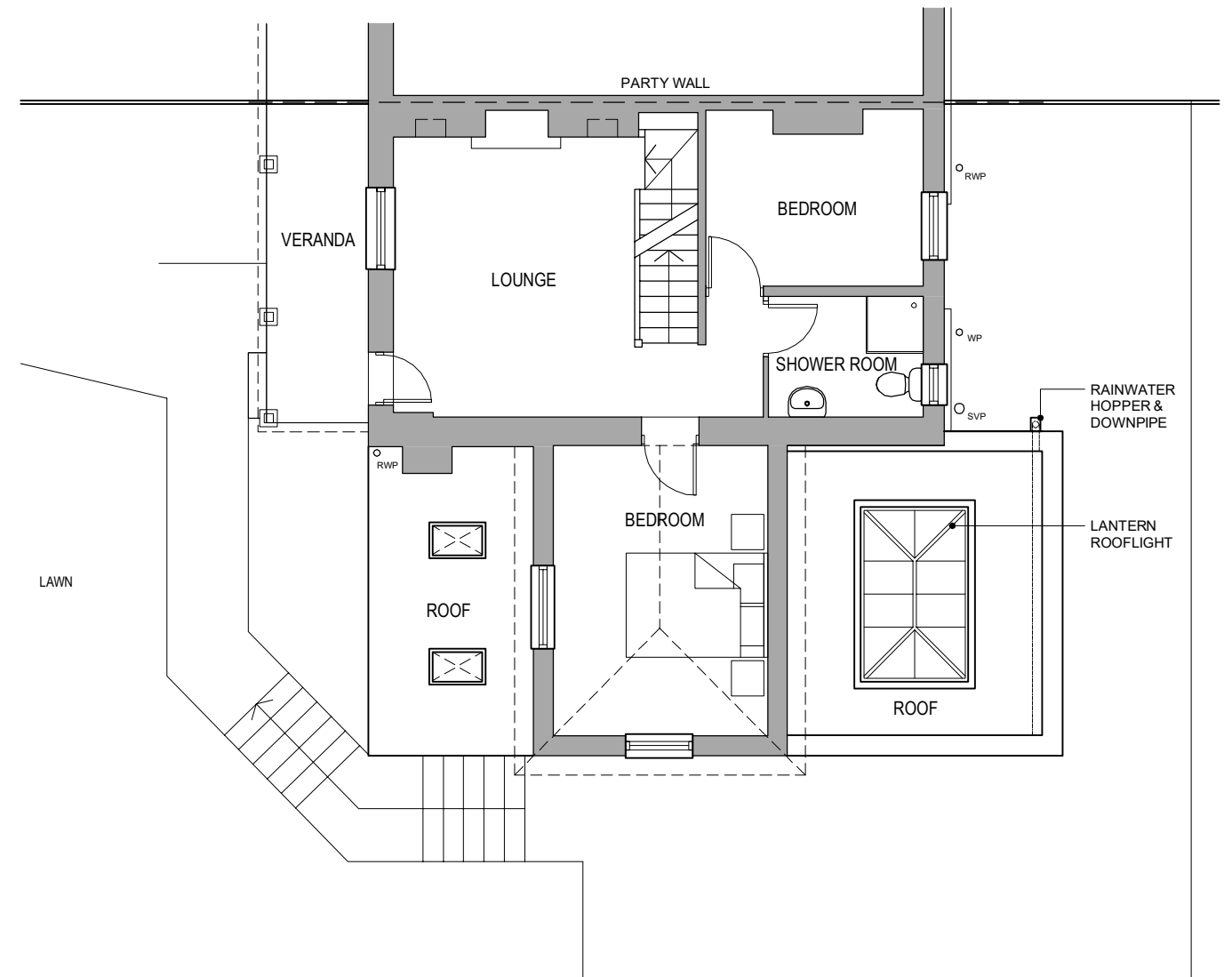
PROPOSED UPPER GROUND FLOOR PLAN
