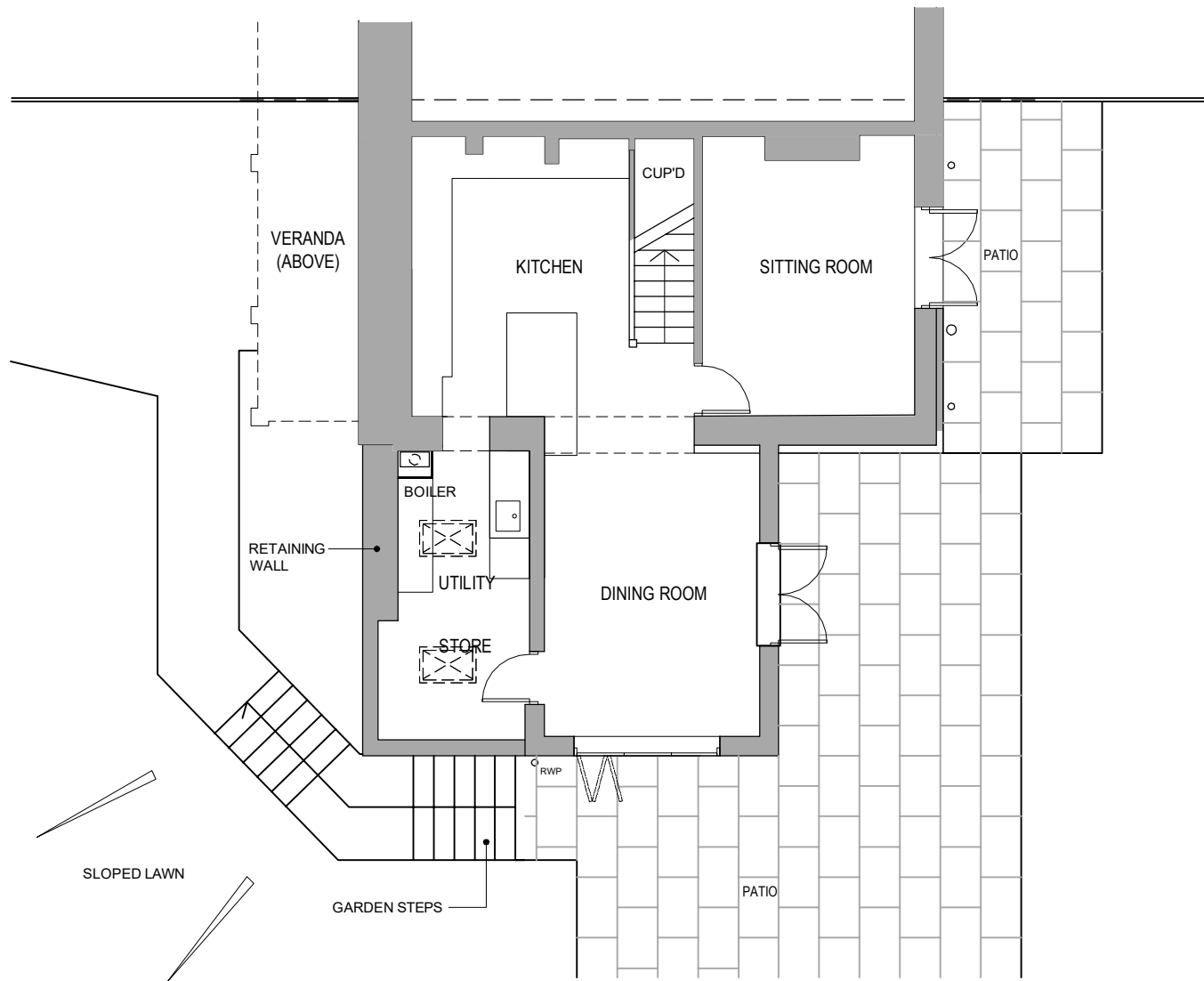
EXISTING LOWER GROUND FLOOR PLAN
