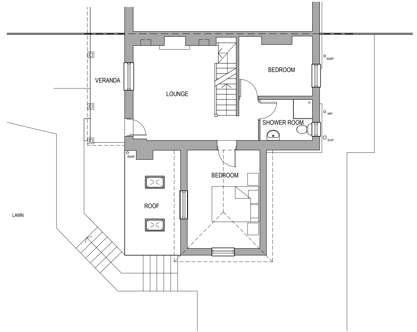
EXISTING UPPER GROUND FLOOR PLAN
