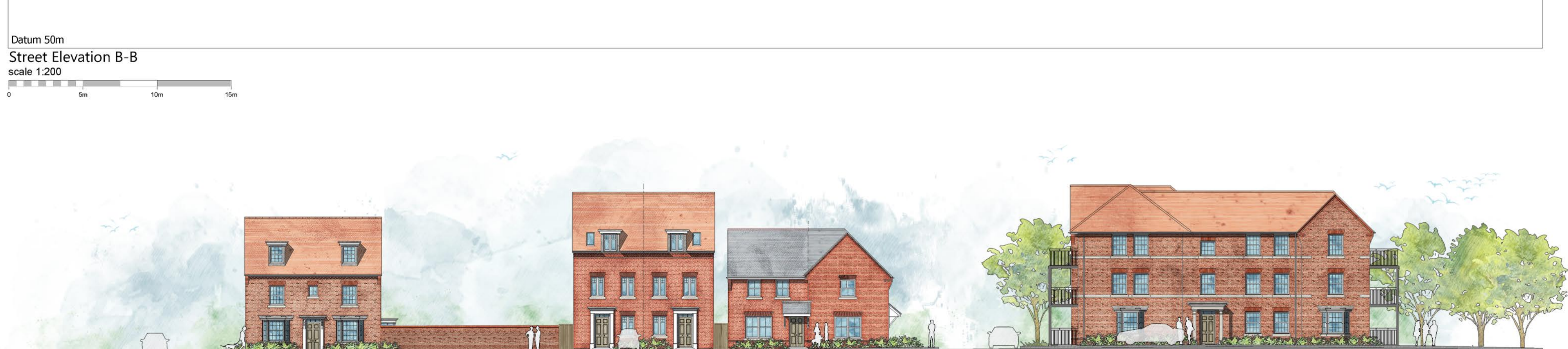
Datum 50m Street Elevation C-C scale 1:200
