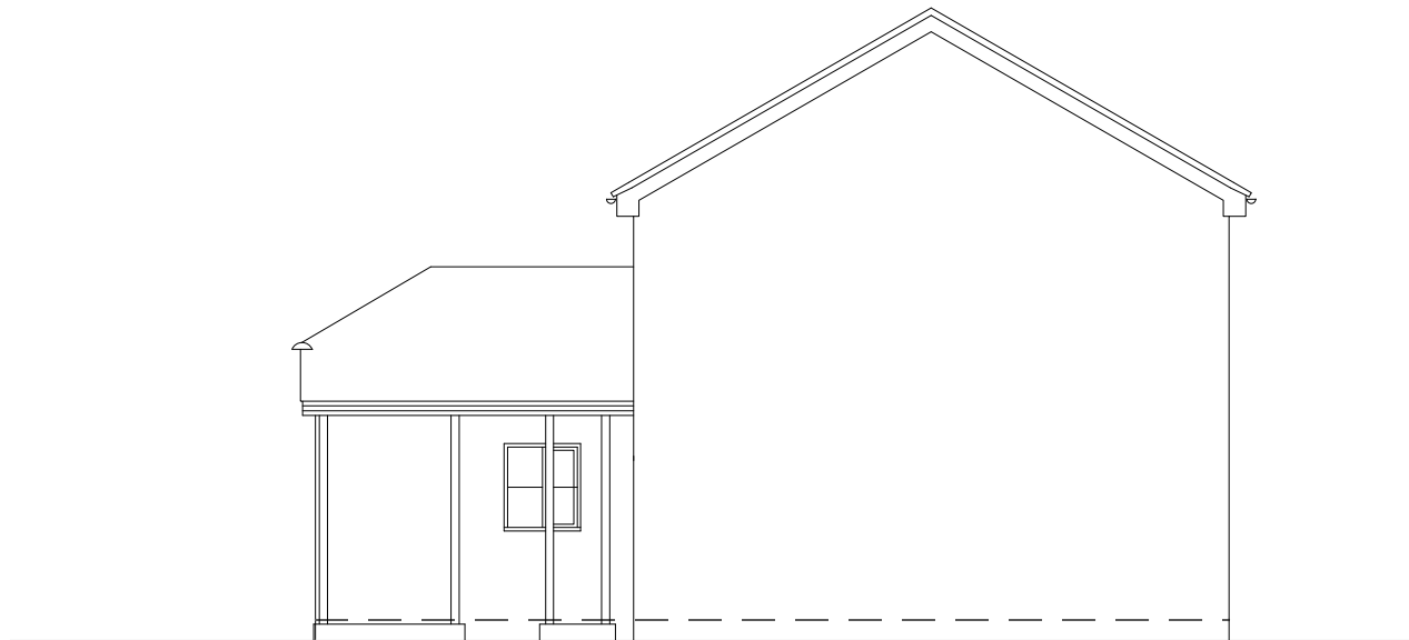
Side Elevation 1 : 100
