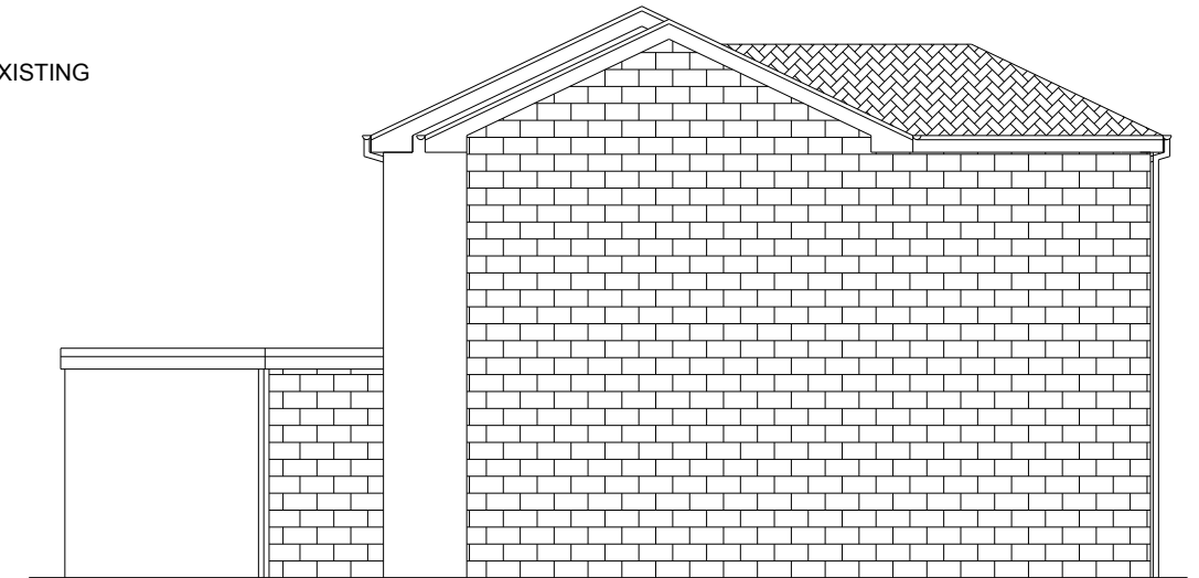
RIGHTSIDE ELEVATION PROPOSED
