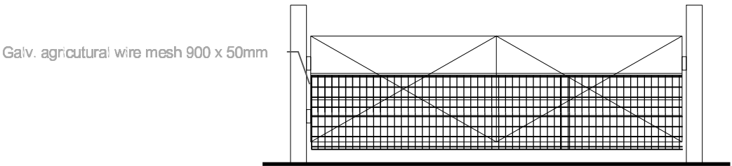
Timber Field Gate Elevation 1:50
