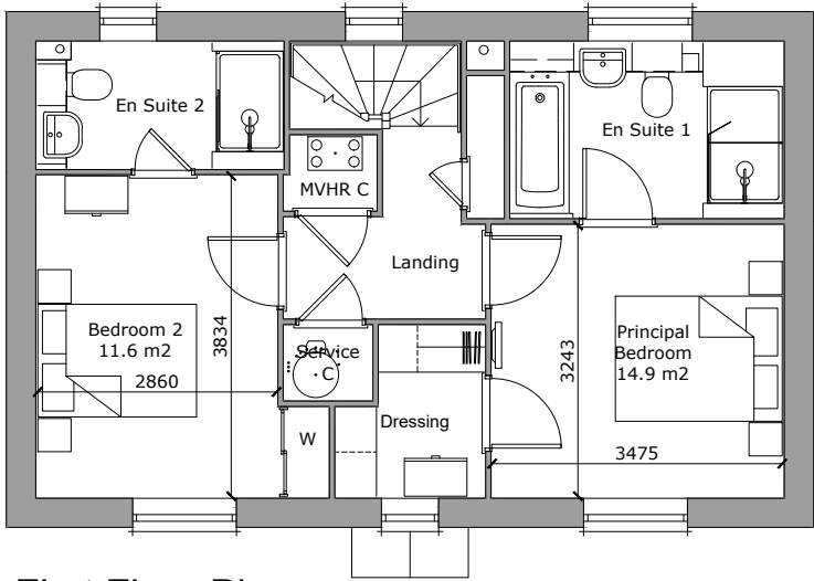
First Floor Plan Area 49.1m²
